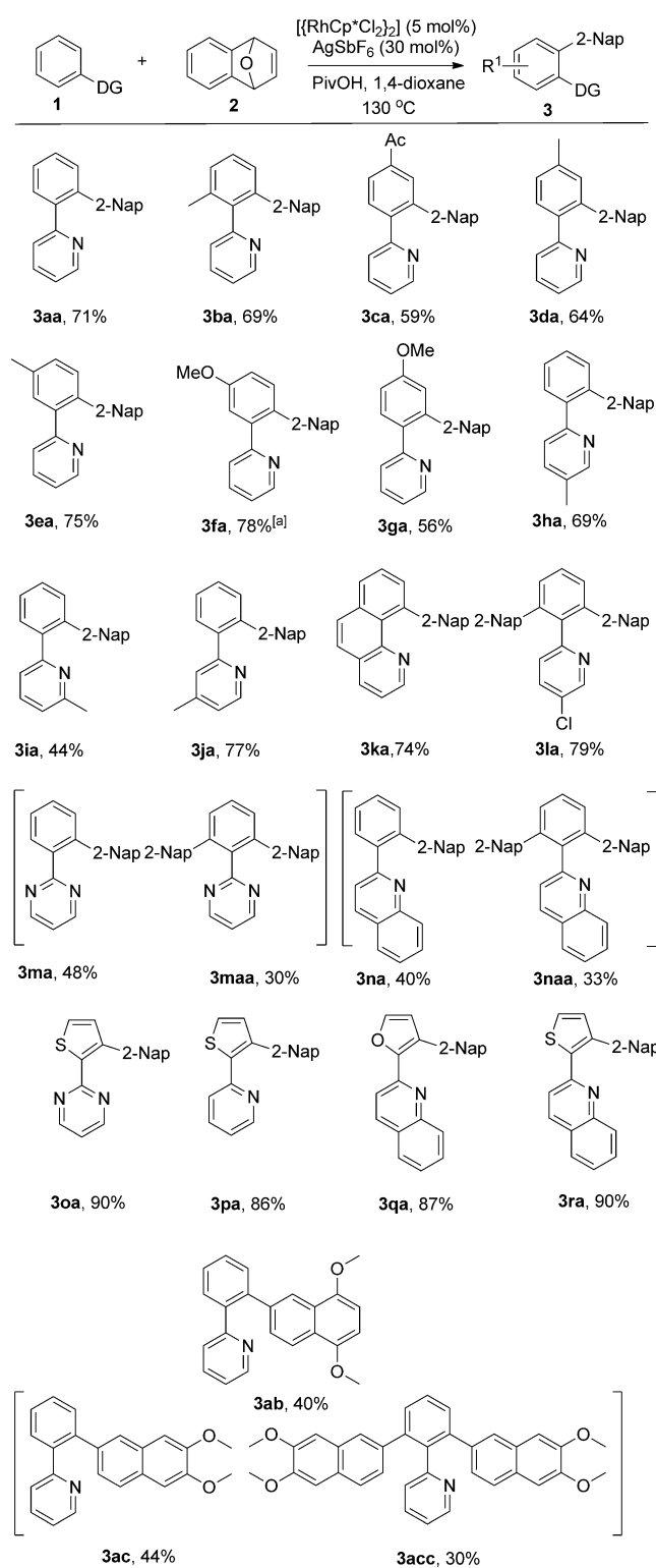
Scheme 2. Dehydative coupling with 7-oxabenzonorbornadienes. Reaction conditions: arene (0.2 mmol), [\{\text{RhCp}^*\text{Cl}_2\}_2] (5 mol %), \text{AgSbF}_6 (30 mol %), \text{PivOH} (0.4 mmol), 7-oxabenzonorbornadiene (0.3 mmol), 1,4-dioxane (2 mL), 130 °C, 24 h. Yield is that of product isolated after column chromatography. [a] Used: arene (0.2 mmol), [\{\text{RhCp}^*(\text{MeCN})_3\}(\text{SbF}_6)_2] (4 mol %), TFA (0.4 mmol), and 7-oxabenzonorbornadiene (0.3 mmol), 1,4-dioxane (2 mL), 130 °C, 24 h. \text{Cp}^* = \text{C}_5\text{Me}_5 , \text{Piv} = \text{pivaloyl} .
